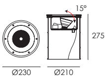
ORIENTABILE / ADJUSTABLE
